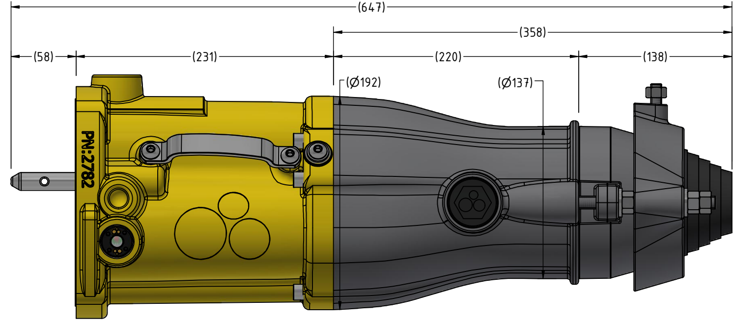
SIDE VIEW
