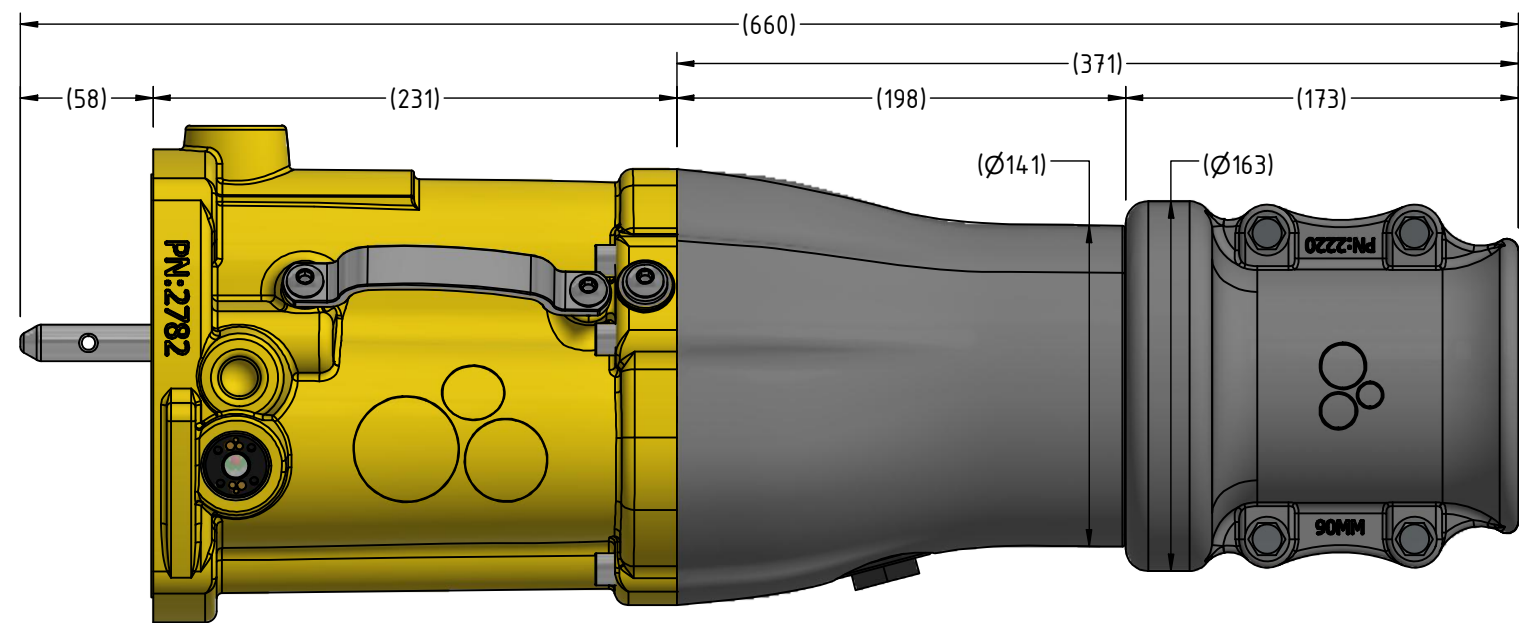
SIDE VIEW
