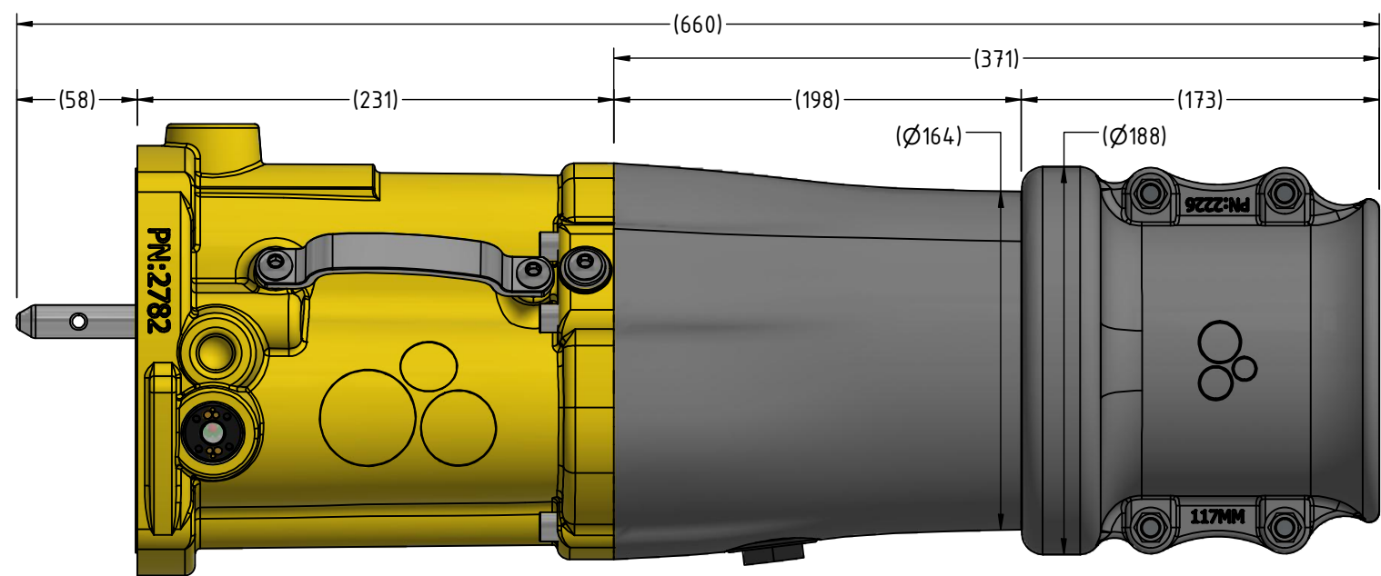
SIDE VIEW
